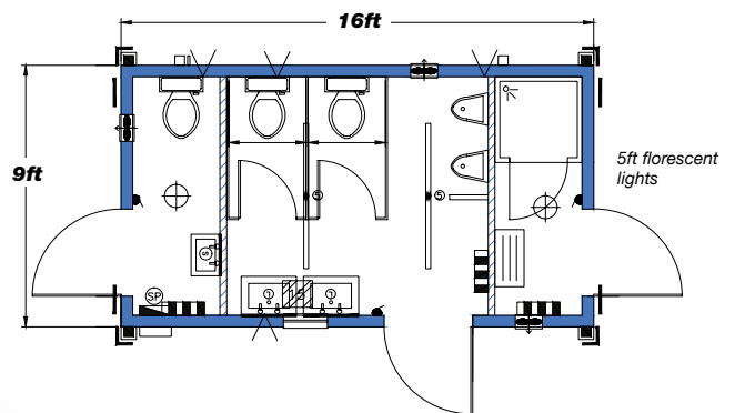
2 + 1 + Shower - 16ft x 9ft
